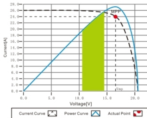
Maximum Power Point Curve
