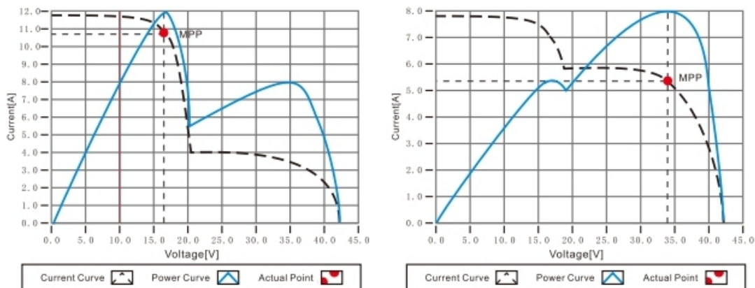
Curves with multiple MPP points
